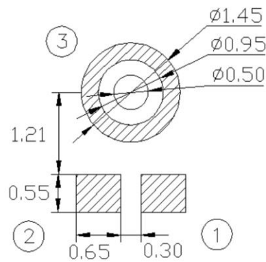
Figure 3. Recommended landing pattern on customers' PCB
