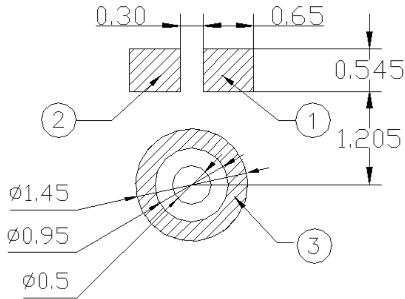
Figure 3. Recommended landing pattern on customers' PCB
