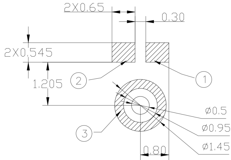
Figure 3. Recommended landing pattern on customers' PCB
