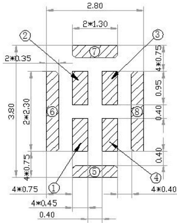
Figure 3. Recommended landing pattern on customers' PCB
