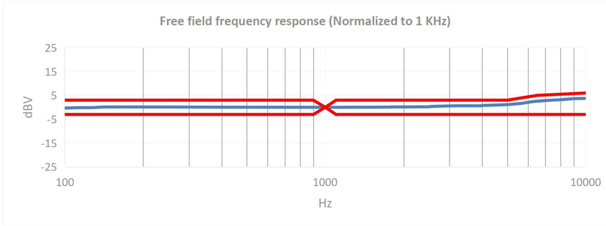
Figure 1. Typical free field frequency response
