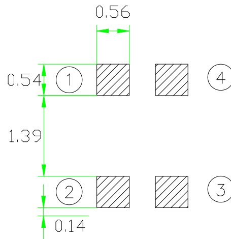
Figure 3. Recommended landing pattern on customers' PCB
