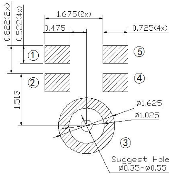
Figure 3. Recommended landing pattern on customers' PCB
