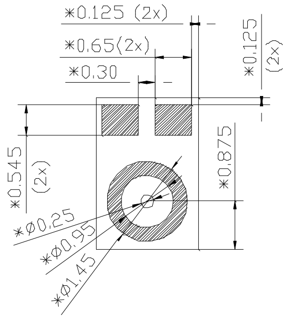
Figure 3. Recommended landing pattern on customers' PCB
